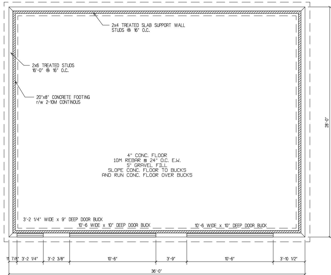
FOUNDATION PLAN
