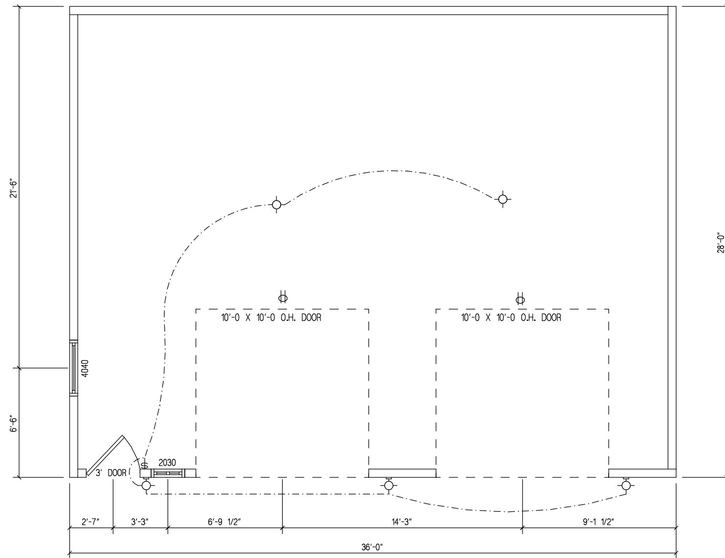
MAIN FLOOR PLAN: 1008 SQ.FT.
